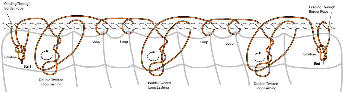
1.25" ProManila lashed to M1250 with #36 Polyester twine
