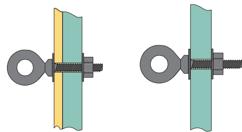
Thru-hole Eyebolt Steel
