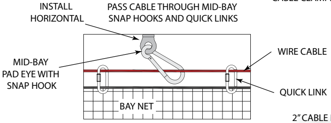
Detail D
