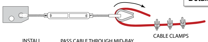
Detail E
